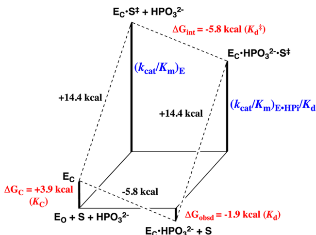
Figure 4. Free energy diagram for the turnover of the truncated substrate glycolaldehyde (S) by free TIM ( E_0 ) and by TIM that is saturated with phosphite dianion [ E_C \cdot HPO_3^{2-} (Scheme 11)] constructed using data from ref 87. The observed tighter binding of phosphite dianion to the transition state complex E_C \cdot S^\ddagger to give E_C \cdot HPO_3^{2-} \cdot S^\ddagger [ \Delta G_{int} = -5.8 kcal/mol (eq 3)] than to the free enzyme E_0 to give E_C \cdot HPO_3^{2-} ( \Delta G_{obsd} = -1.9 kcal/mol) represents the “interaction energy” of 3.9 kcal/mol. 90 This can be attributed to a \Delta G_c of 3.9 kcal/mol for the unfavorable conformational change that converts the inactive open ground state enzyme E_0 to the active closed enzyme E_C (eq 4). The observed \Delta G^\ddagger value of 18.3 kcal/mol for the turnover of glycolaldehyde with second-order rate constant (k_{cat}/K_m)_E can be partitioned into a \Delta G^\ddagger of 14.4 kcal/mol for the transfer of a proton from glycolaldehyde to E_C and a \Delta G_c of 3.9 kcal/mol for the unfavorable conformational change that converts E_0 to E_C .
