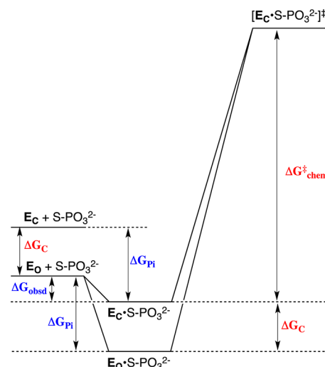
Figure 6. Free energy profile for the reaction of a whole phosphorylated substrate \text{S-PO}_3^{2-} catalyzed by an enzyme that exists predominantly in a stable inactive open form, \text{E}_\text{O} . For the sake of simplicity, only the binding energy of the phosphodianion portion of the substrate, \Delta G_{\text{Pi}} , is shown. The relatively small observed binding energy of the phosphodianion group ( \Delta G_{\text{obsd}} ) is the sum of the much larger total available binding energy of this group ( \Delta G_{\text{Pi}} ) and the binding energy that is utilized to drive the unfavorable enzyme conformational change ( \Delta G_\text{C} ). Catalysis occurs at a higher-energy active closed form \text{E}_\text{C} , which is stabilized by interactions with the phosphodianion group of the substrate at the \text{E}_\text{C}\cdot\text{S-PO}_3^{2-} Michaelis complex (top profile). For the case in which the phosphodianion binding energy is not used to drive the unfavorable conformational change at the ground state Michaelis complex (bottom profile), the activation barrier \Delta G^\ddagger_{\text{chem}} for turnover of the enzyme-bound substrate will increase by an amount \Delta G_\text{C} (see the text).
